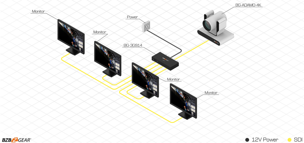
BG-3GS14 Connection Diagram
